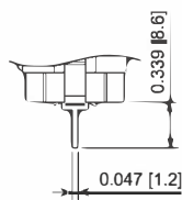
PCB Pin
