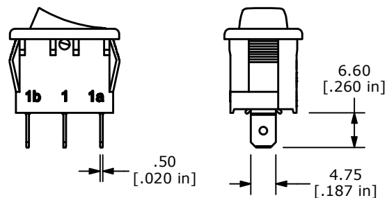
"G" TERMINAL
