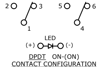
DPDT LED SCHEMATIC
