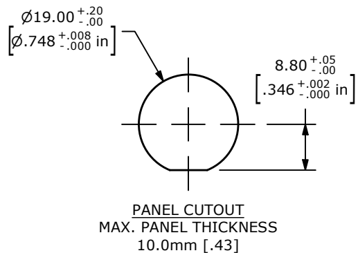
PANEL CUTOUT
